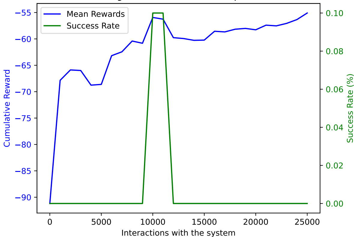
PPO on AWAKE with DoF: 5 and trained on 25000 samples averaged over 10 validation episodes
