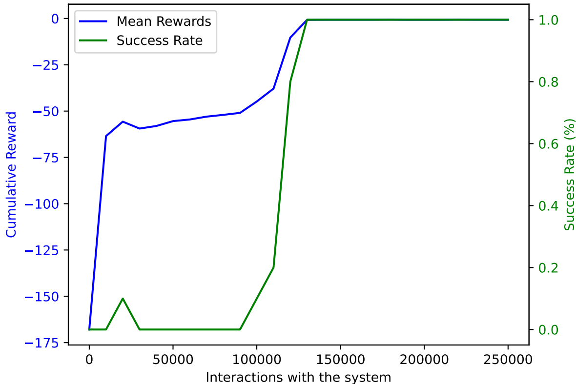
PPO on AWAKE with DoF: 5 and trained on 250000 samples averaged over 10 validation episodes
