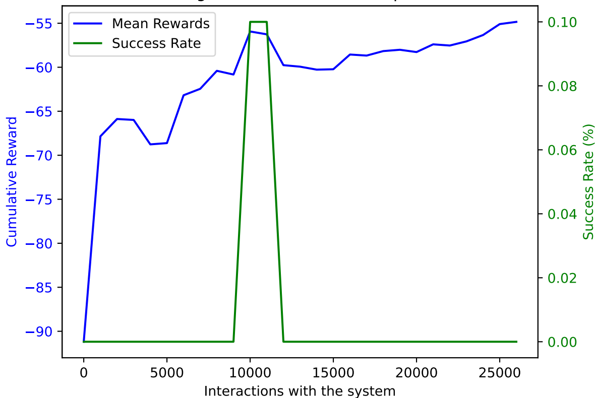
PPO on AWAKE with DoF: 5 and trained on 26000 samples averaged over 10 validation episodes
