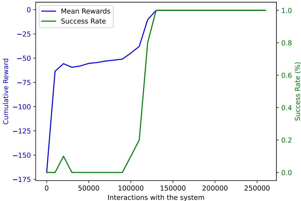
PPO on AWAKE with DoF: 5 and trained on 260000 samples averaged over 10 validation episodes
