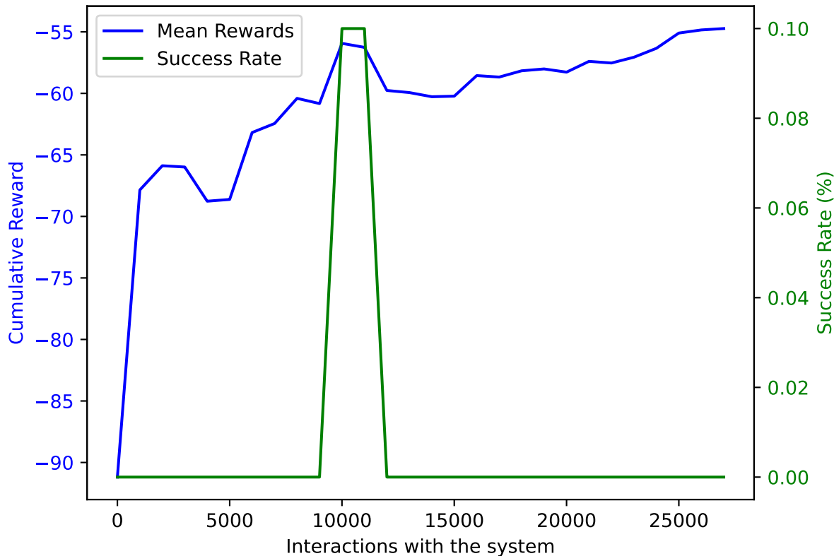
PPO on AWAKE with DoF: 5 and trained on 27000 samples averaged over 10 validation episodes
