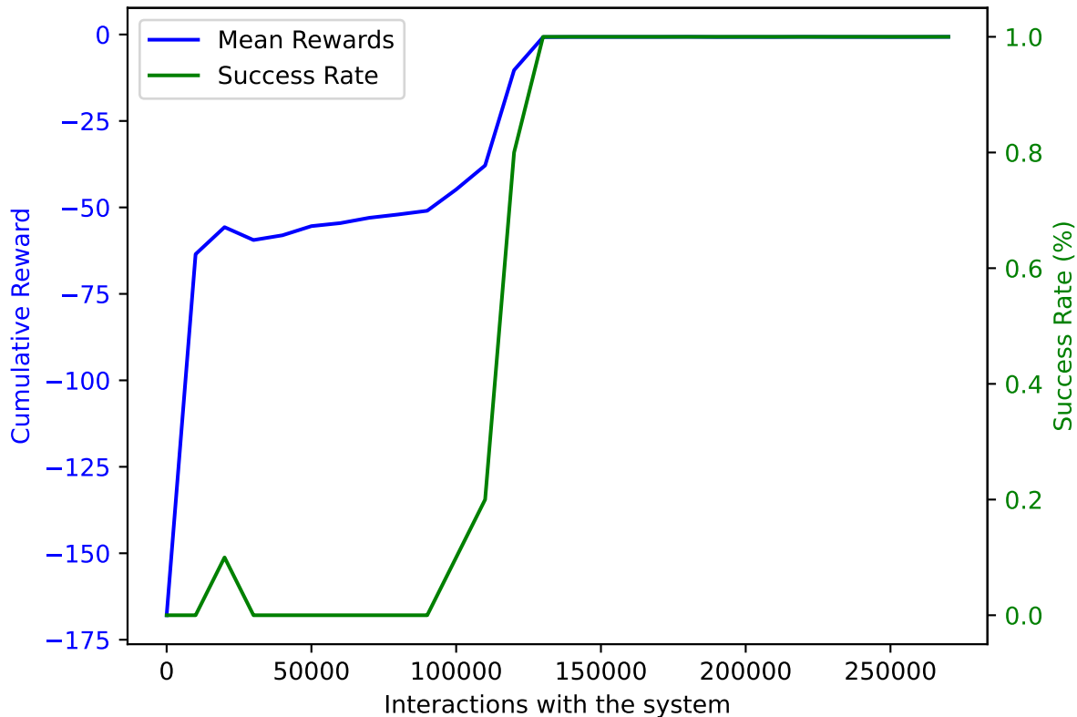
PPO on AWAKE with DoF: 5 and trained on 270000 samples averaged over 10 validation episodes
