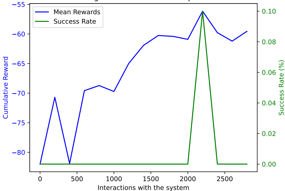
PPO on AWAKE with DoF: 5 and trained on 2800 samples averaged over 10 validation episodes
