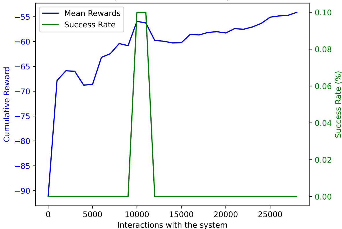
PPO on AWAKE with DoF: 5 and trained on 28000 samples averaged over 10 validation episodes
