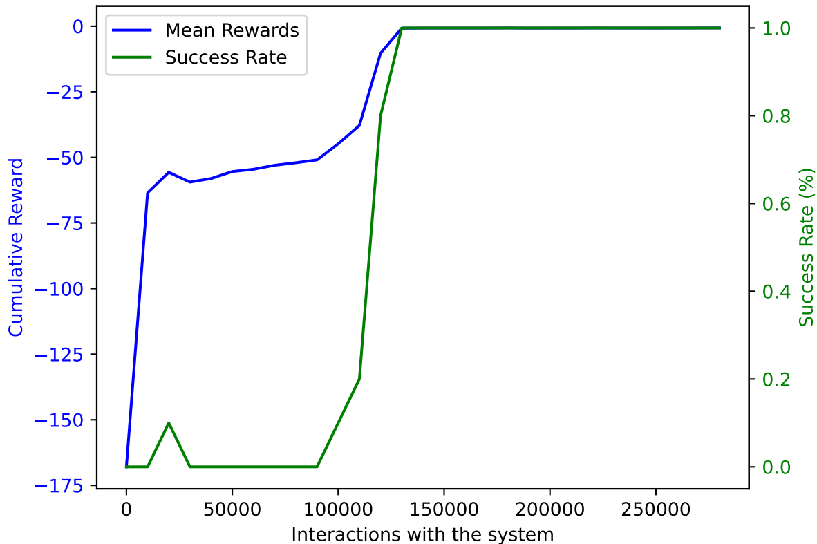
PPO on AWAKE with DoF: 5 and trained on 280000 samples averaged over 10 validation episodes
