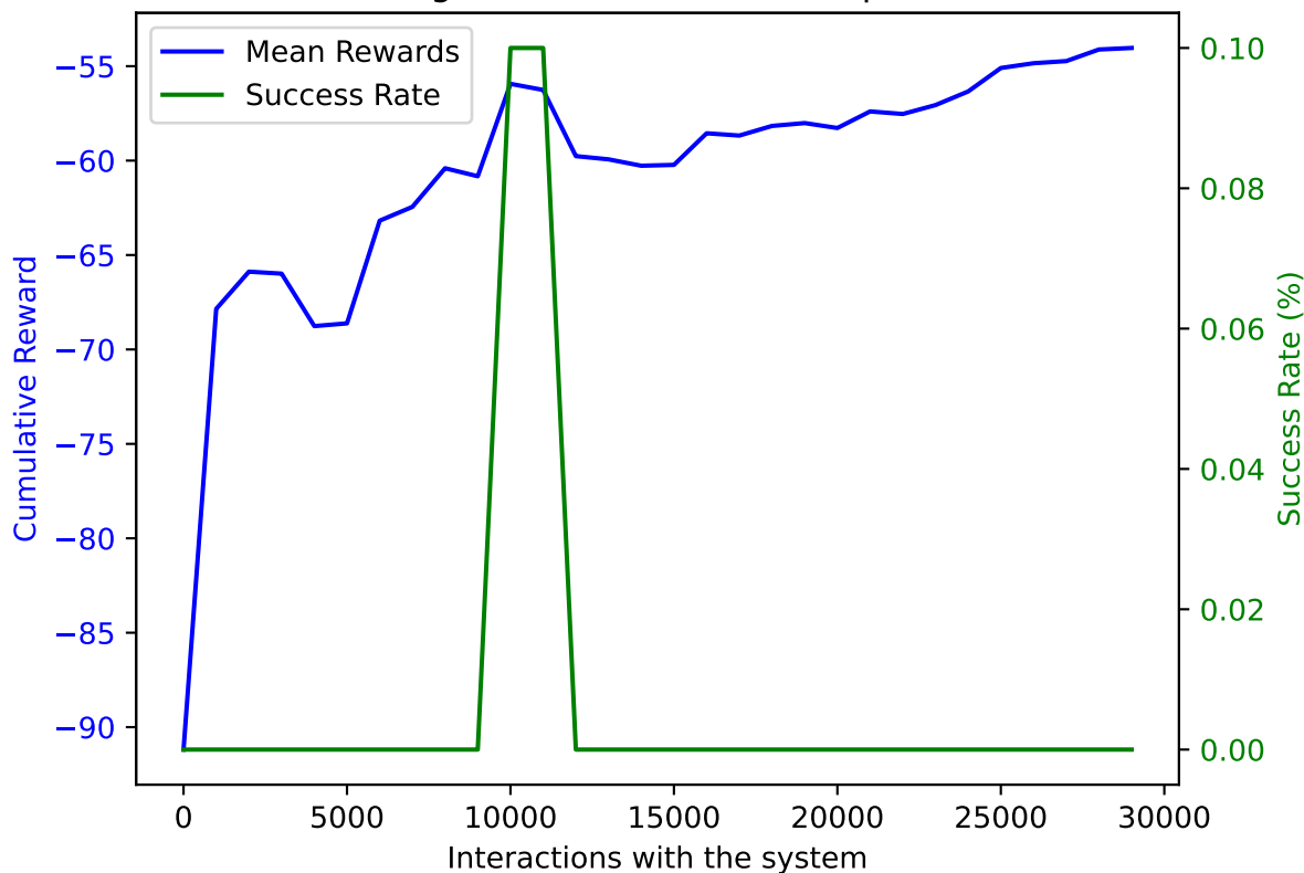
PPO on AWAKE with DoF: 5 and trained on 29000 samples averaged over 10 validation episodes
