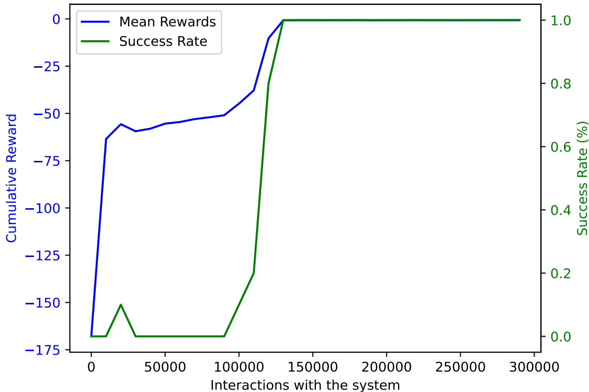
PPO on AWAKE with DoF: 5 and trained on 290000 samples averaged over 10 validation episodes
