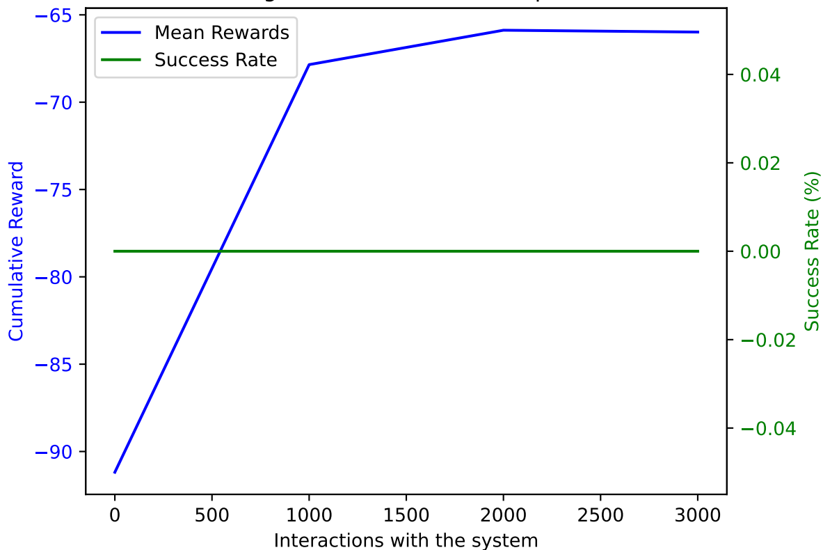
PPO on AWAKE with DoF: 5 and trained on 3000 samples averaged over 10 validation episodes
