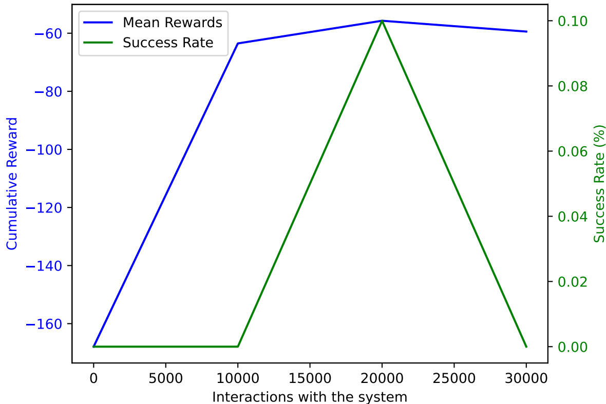
PPO on AWAKE with DoF: 5 and trained on 30000 samples averaged over 10 validation episodes
