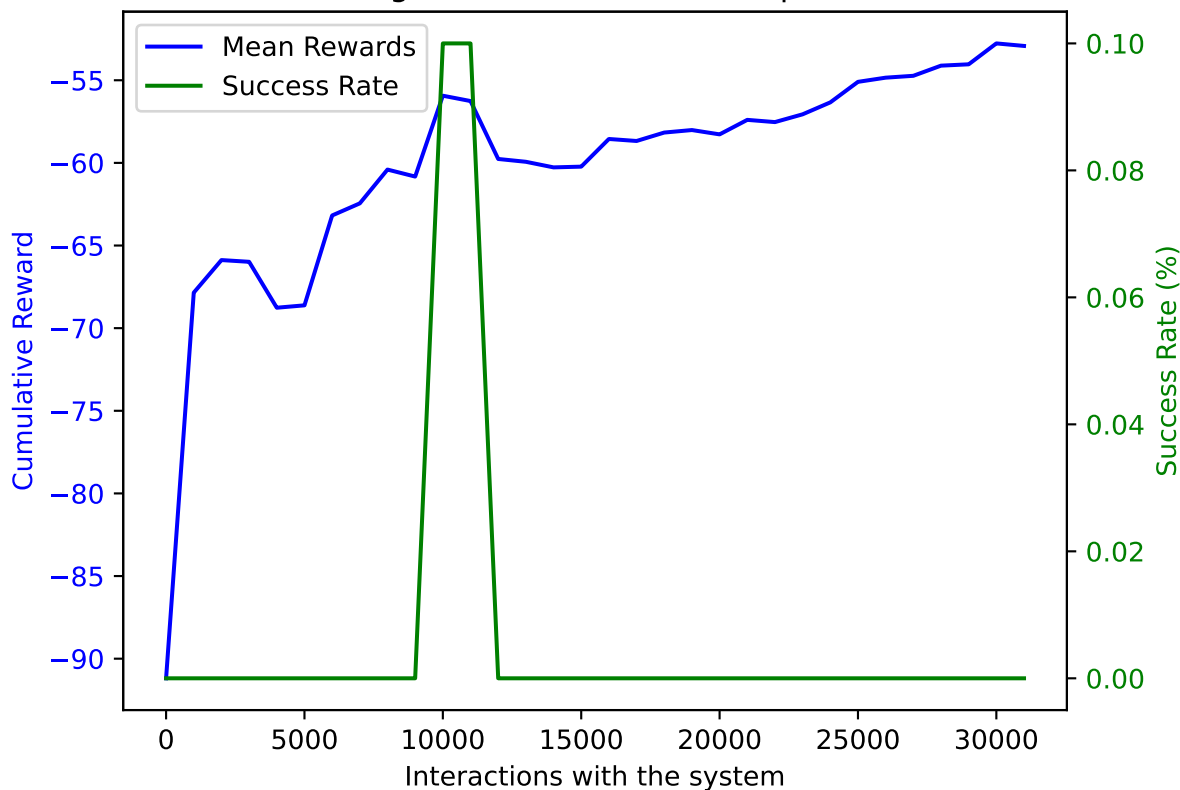
PPO on AWAKE with DoF: 5 and trained on 31000 samples averaged over 10 validation episodes
