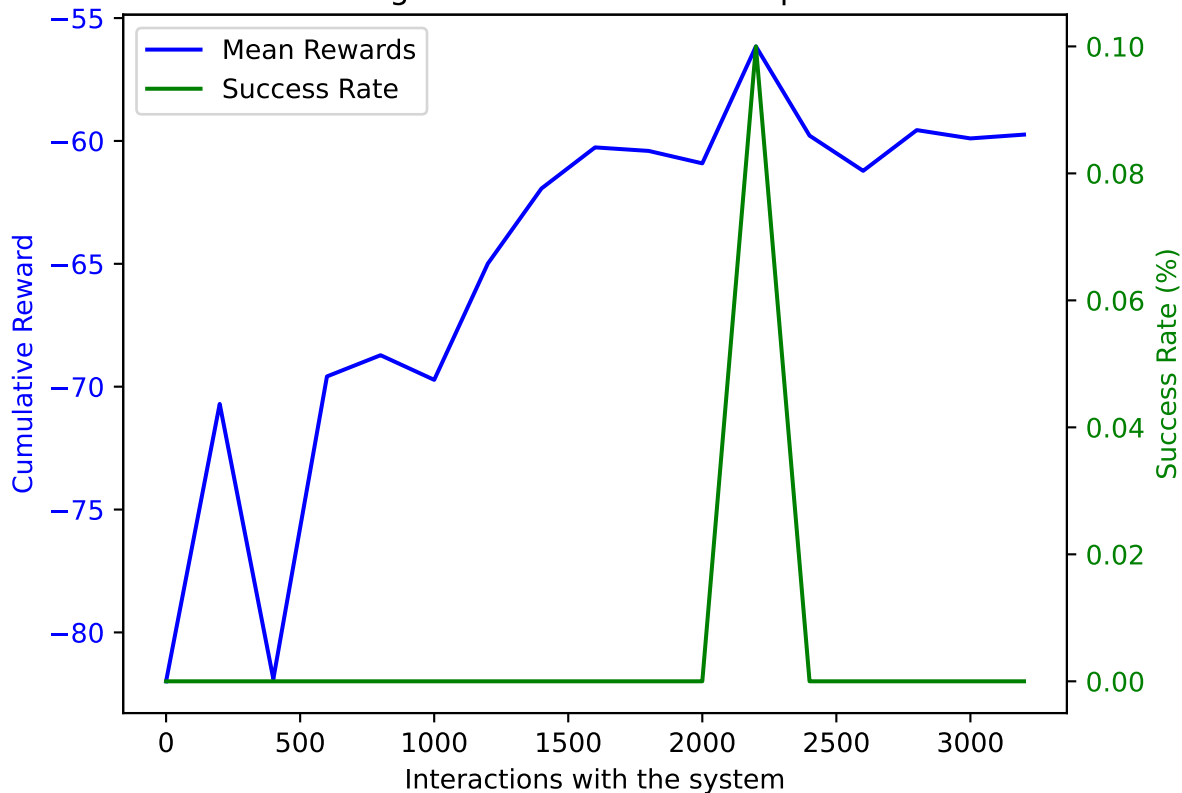
PPO on AWAKE with DoF: 5 and trained on 3200 samples averaged over 10 validation episodes
