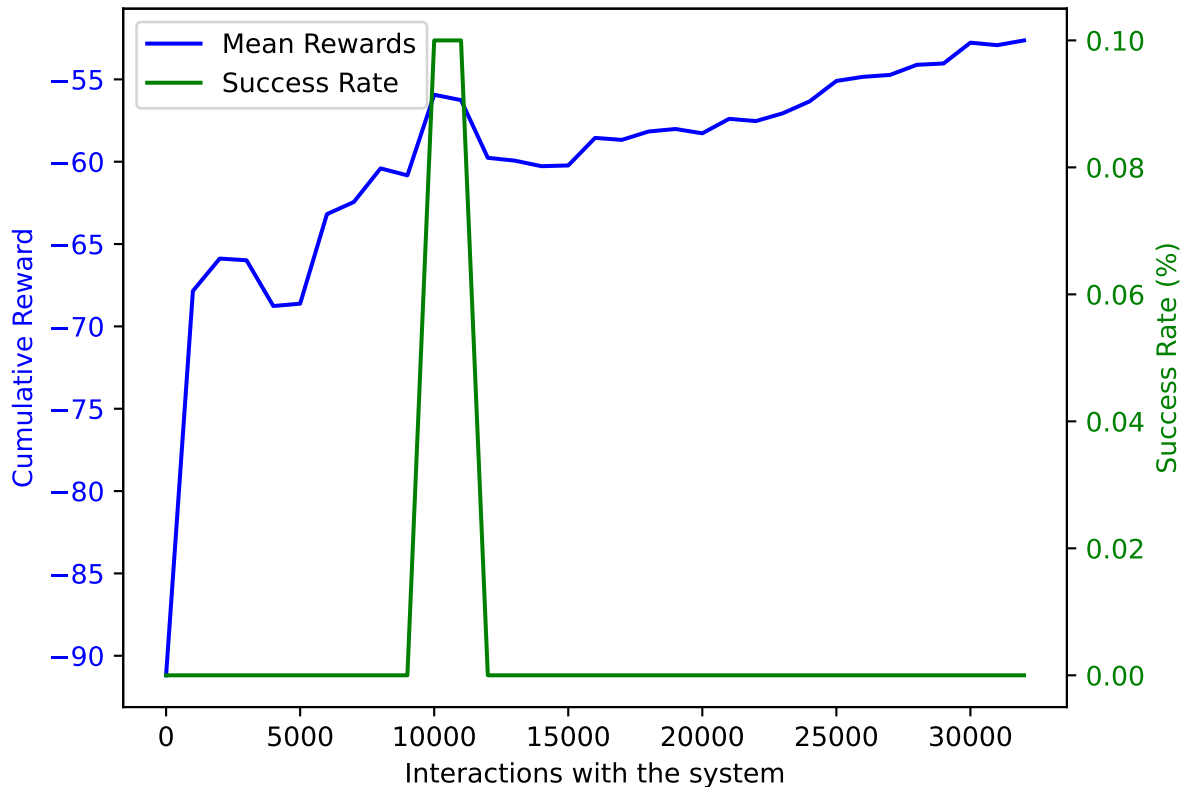
PPO on AWAKE with DoF: 5 and trained on 32000 samples averaged over 10 validation episodes
