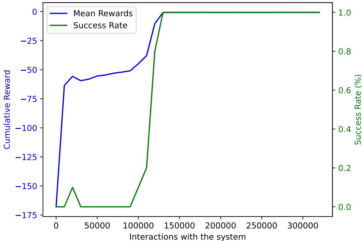
PPO on AWAKE with DoF: 5 and trained on 320000 samples averaged over 10 validation episodes
