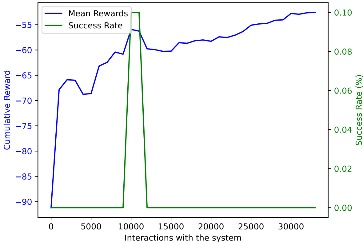
PPO on AWAKE with DoF: 5 and trained on 33000 samples averaged over 10 validation episodes
