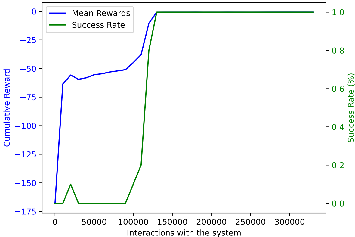
PPO on AWAKE with DoF: 5 and trained on 330000 samples averaged over 10 validation episodes
