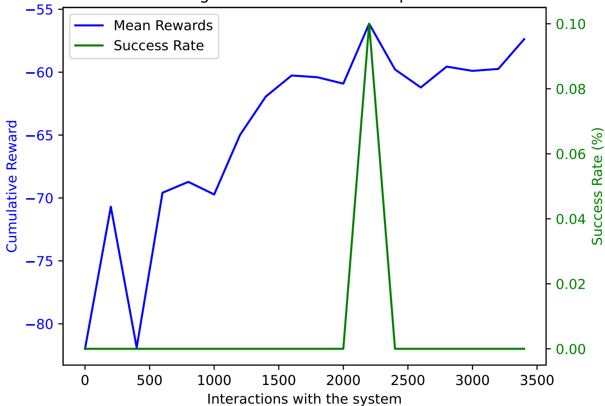
PPO on AWAKE with DoF: 5 and trained on 3400 samples averaged over 10 validation episodes
