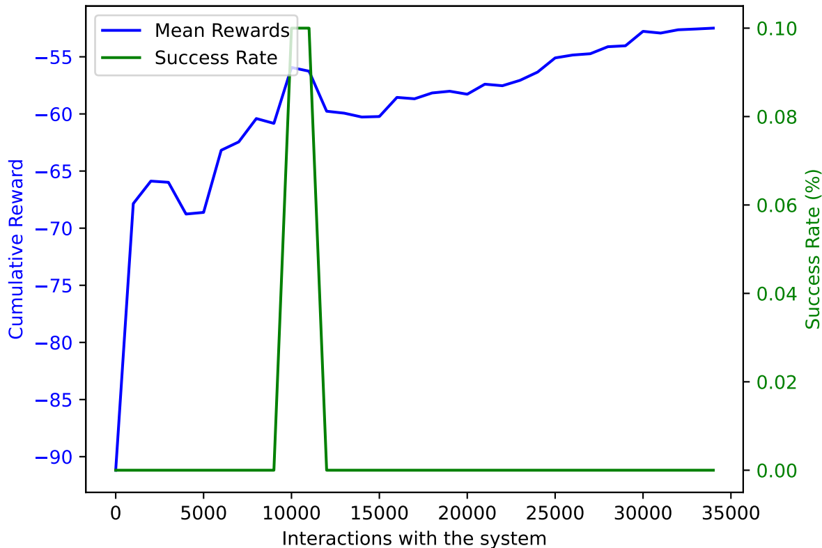
PPO on AWAKE with DoF: 5 and trained on 34000 samples averaged over 10 validation episodes
