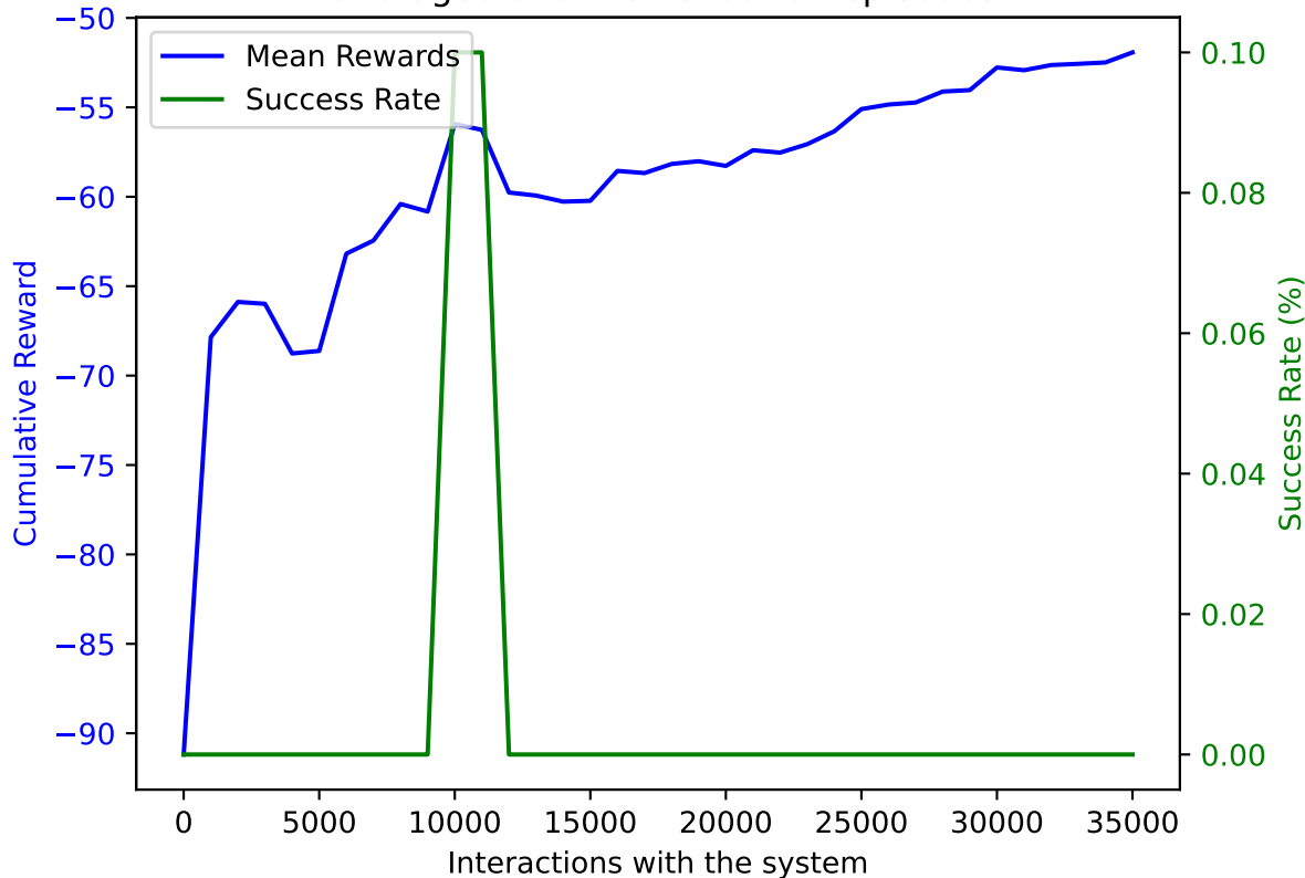
PPO on AWAKE with DoF: 5 and trained on 35000 samples averaged over 10 validation episodes
