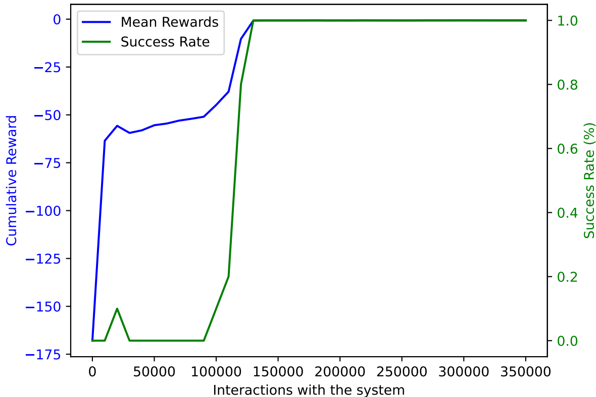
PPO on AWAKE with DoF: 5 and trained on 350000 samples averaged over 10 validation episodes
