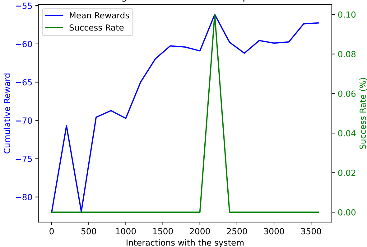
PPO on AWAKE with DoF: 5 and trained on 3600 samples averaged over 10 validation episodes
