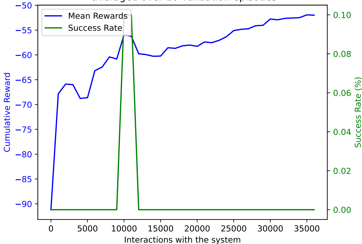
PPO on AWAKE with DoF: 5 and trained on 36000 samples averaged over 10 validation episodes
