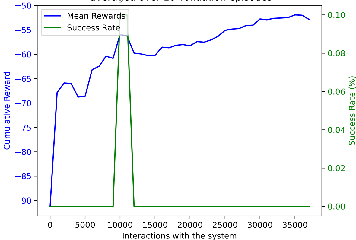
PPO on AWAKE with DoF: 5 and trained on 37000 samples averaged over 10 validation episodes
