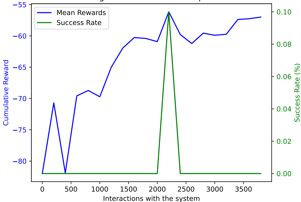
PPO on AWAKE with DoF: 5 and trained on 3800 samples averaged over 10 validation episodes
