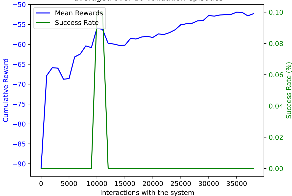
PPO on AWAKE with DoF: 5 and trained on 38000 samples averaged over 10 validation episodes
