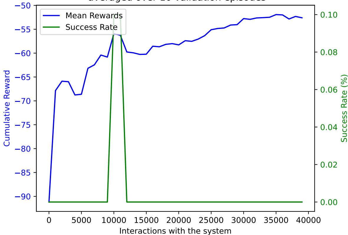
PPO on AWAKE with DoF: 5 and trained on 39000 samples averaged over 10 validation episodes
