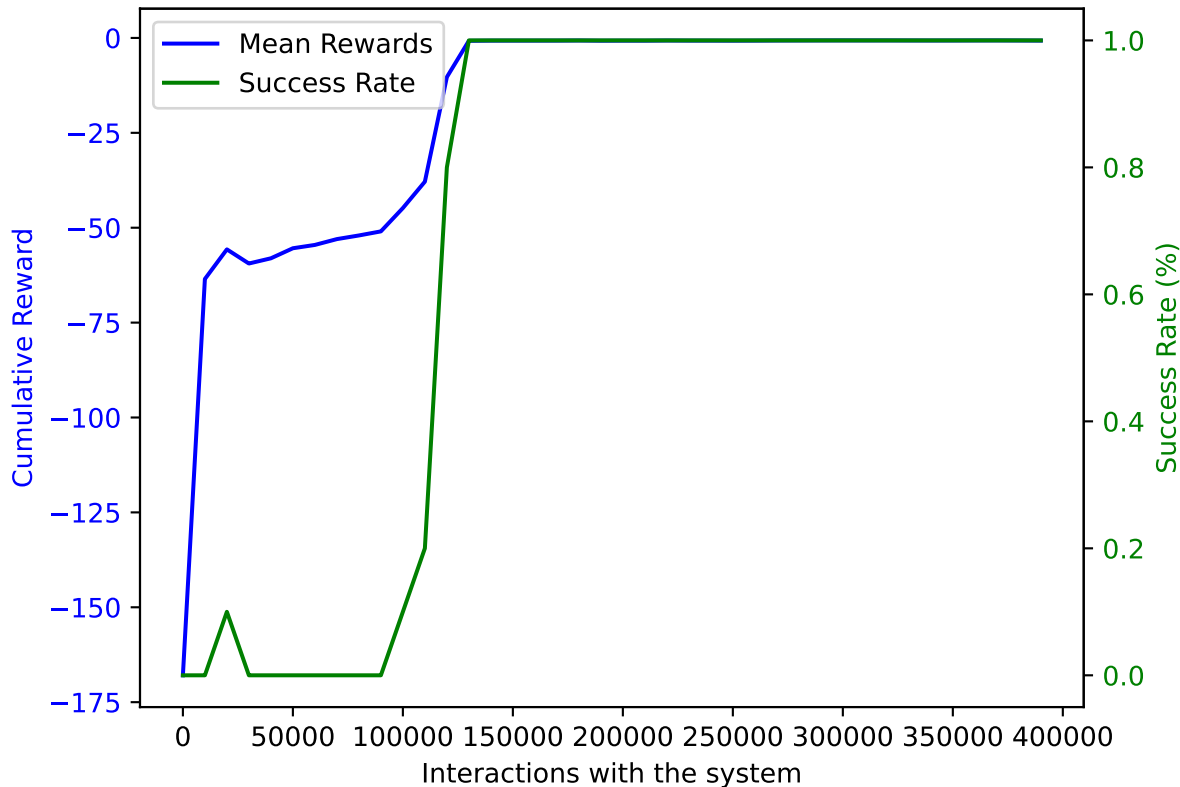
PPO on AWAKE with DoF: 5 and trained on 390000 samples averaged over 10 validation episodes
