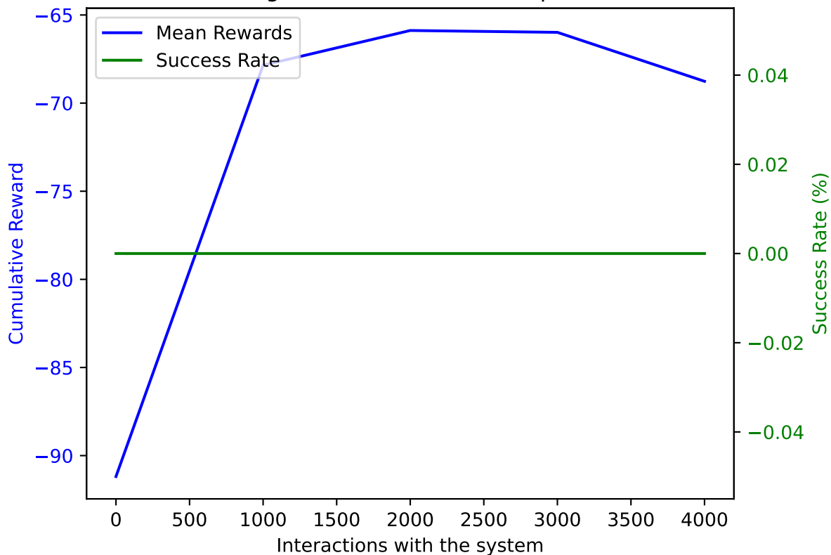
PPO on AWAKE with DoF: 5 and trained on 4000 samples averaged over 10 validation episodes
