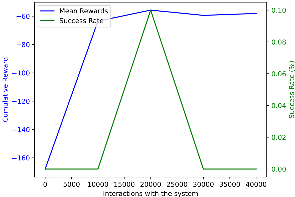
PPO on AWAKE with DoF: 5 and trained on 40000 samples averaged over 10 validation episodes
