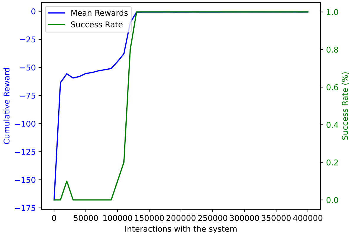
PPO on AWAKE with DoF: 5 and trained on 400000 samples averaged over 10 validation episodes
