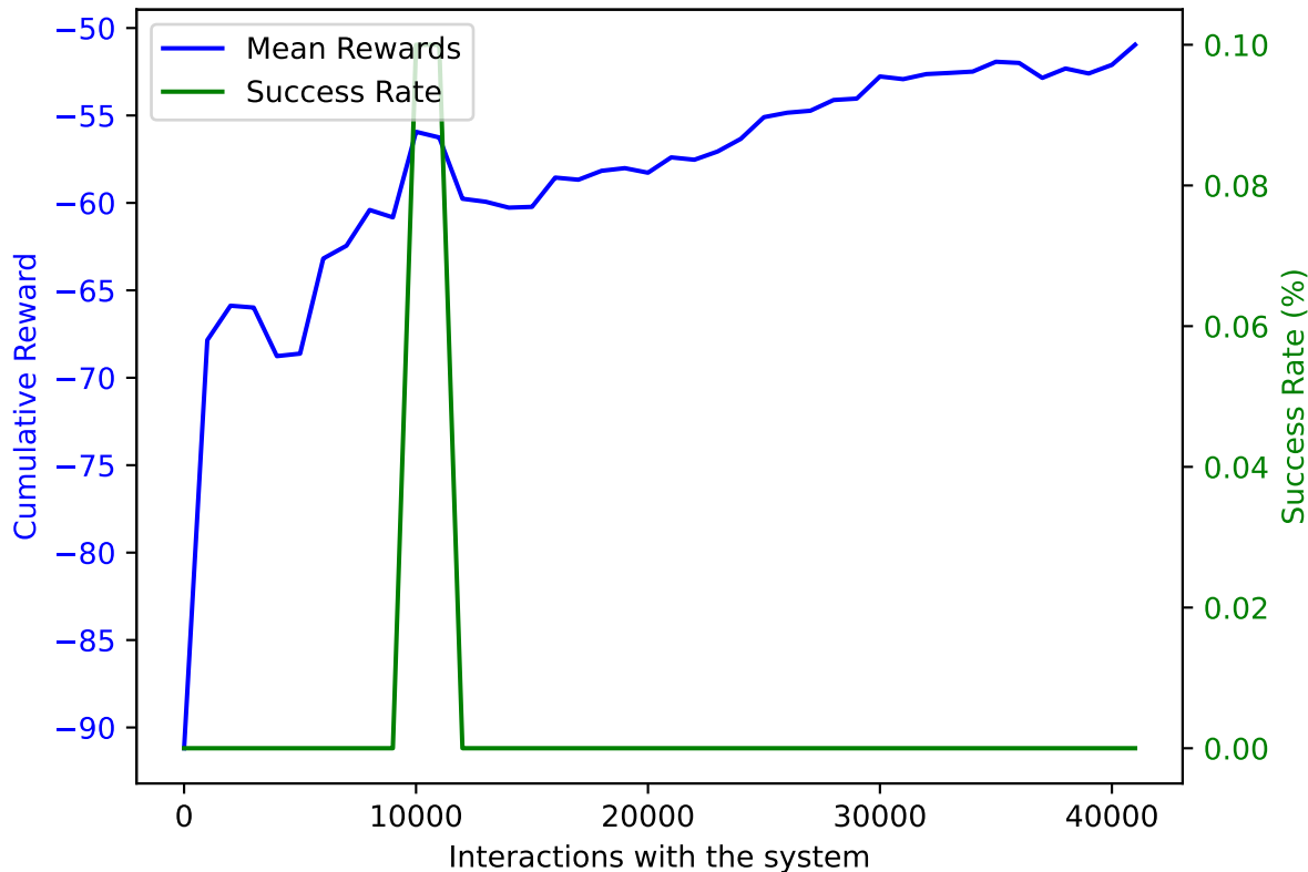
PPO on AWAKE with DoF: 5 and trained on 41000 samples averaged over 10 validation episodes
