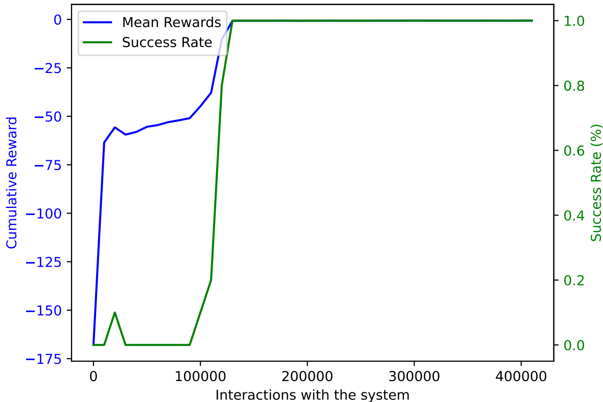
PPO on AWAKE with DoF: 5 and trained on 410000 samples averaged over 10 validation episodes
