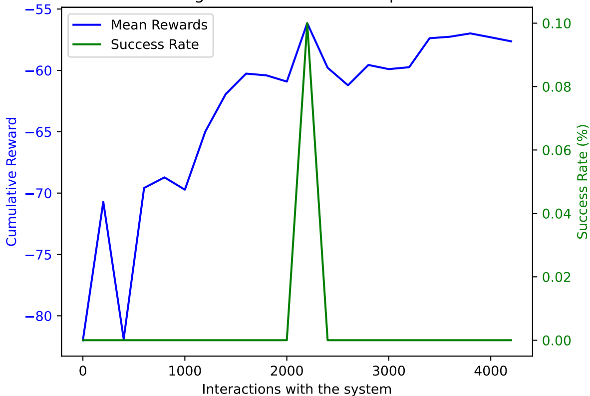
PPO on AWAKE with DoF: 5 and trained on 4200 samples averaged over 10 validation episodes
