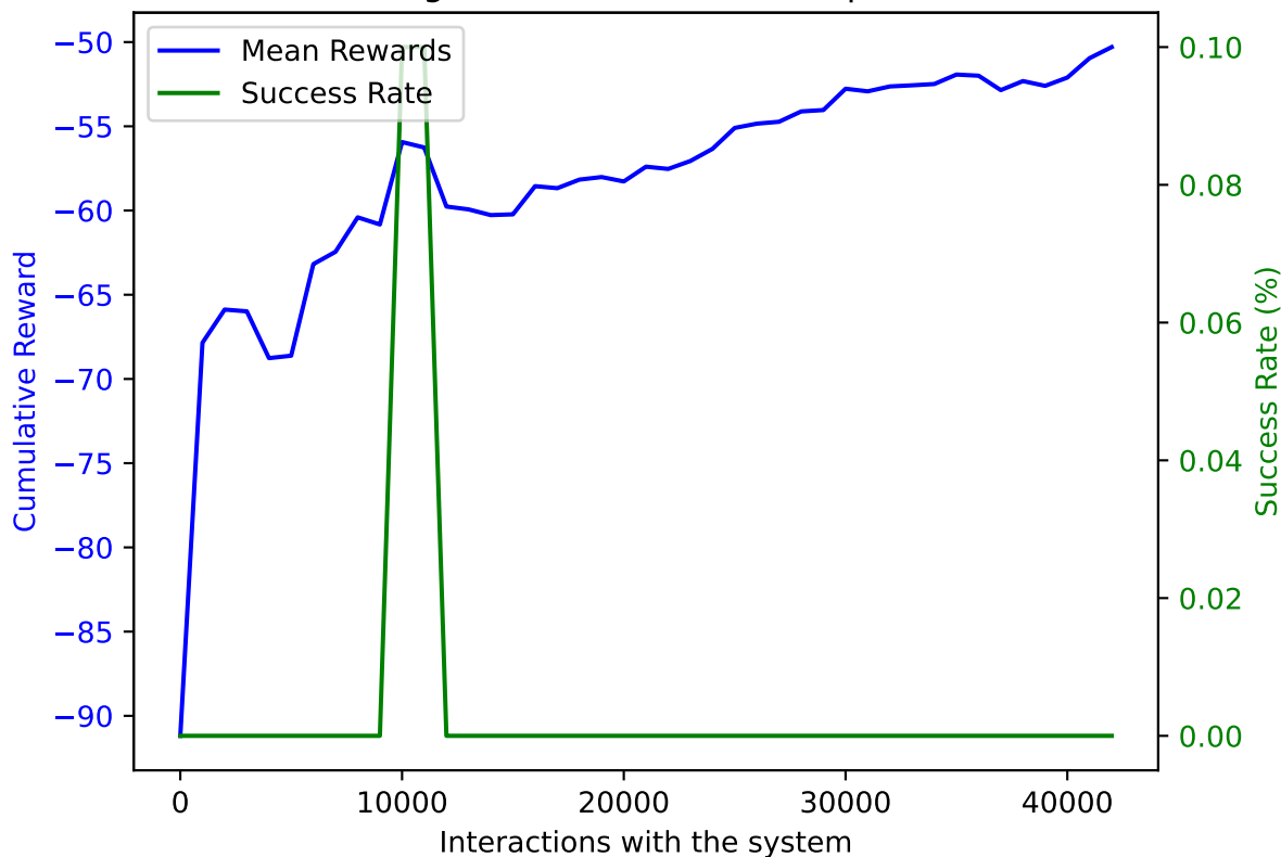
PPO on AWAKE with DoF: 5 and trained on 42000 samples averaged over 10 validation episodes
