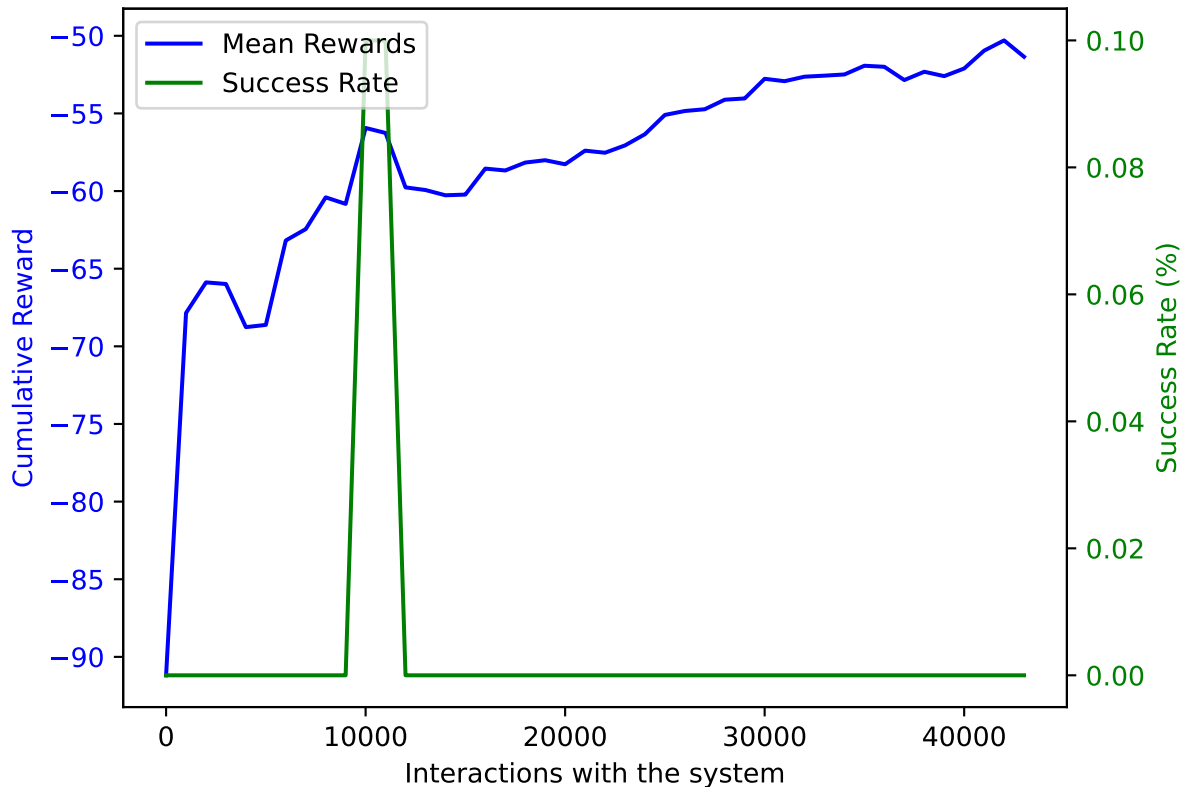
PPO on AWAKE with DoF: 5 and trained on 43000 samples averaged over 10 validation episodes
