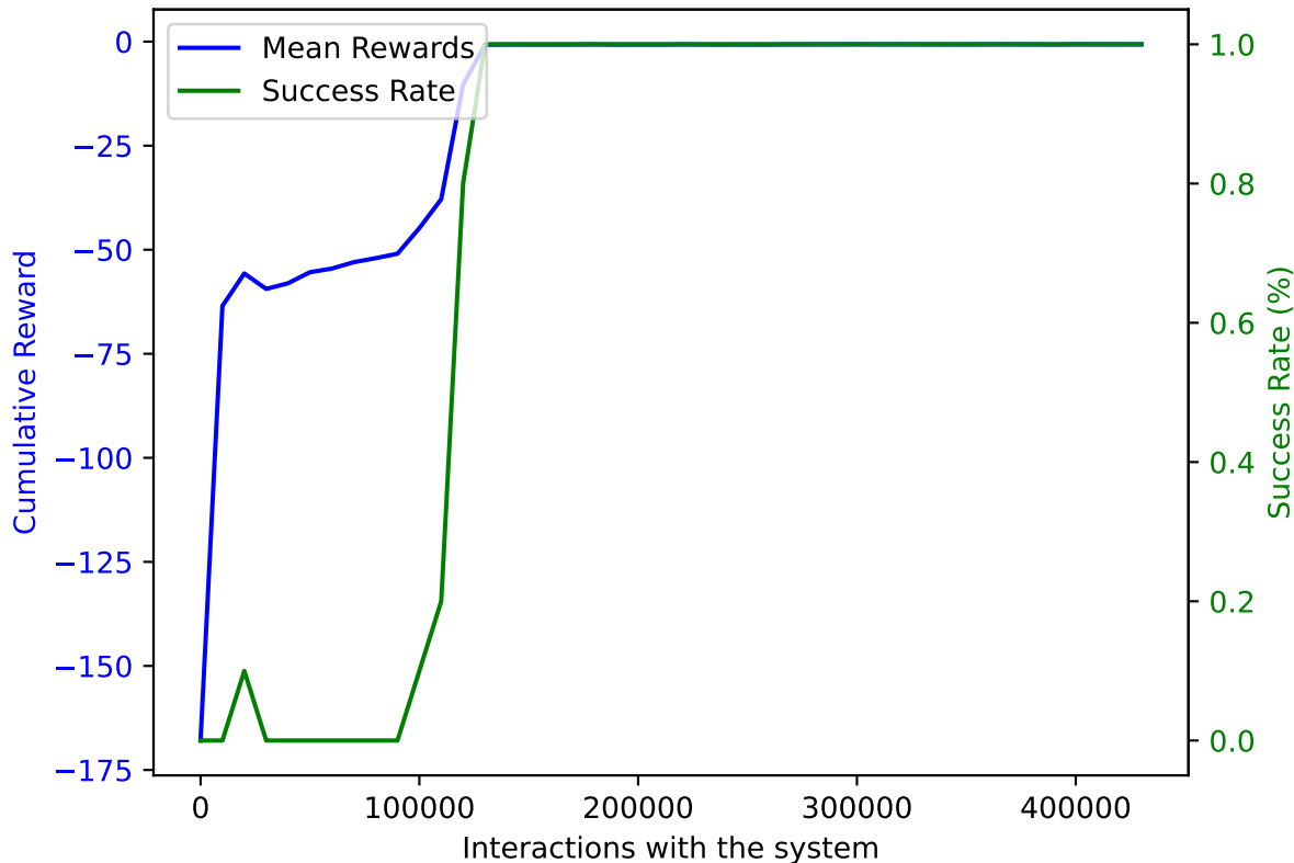
PPO on AWAKE with DoF: 5 and trained on 430000 samples averaged over 10 validation episodes
