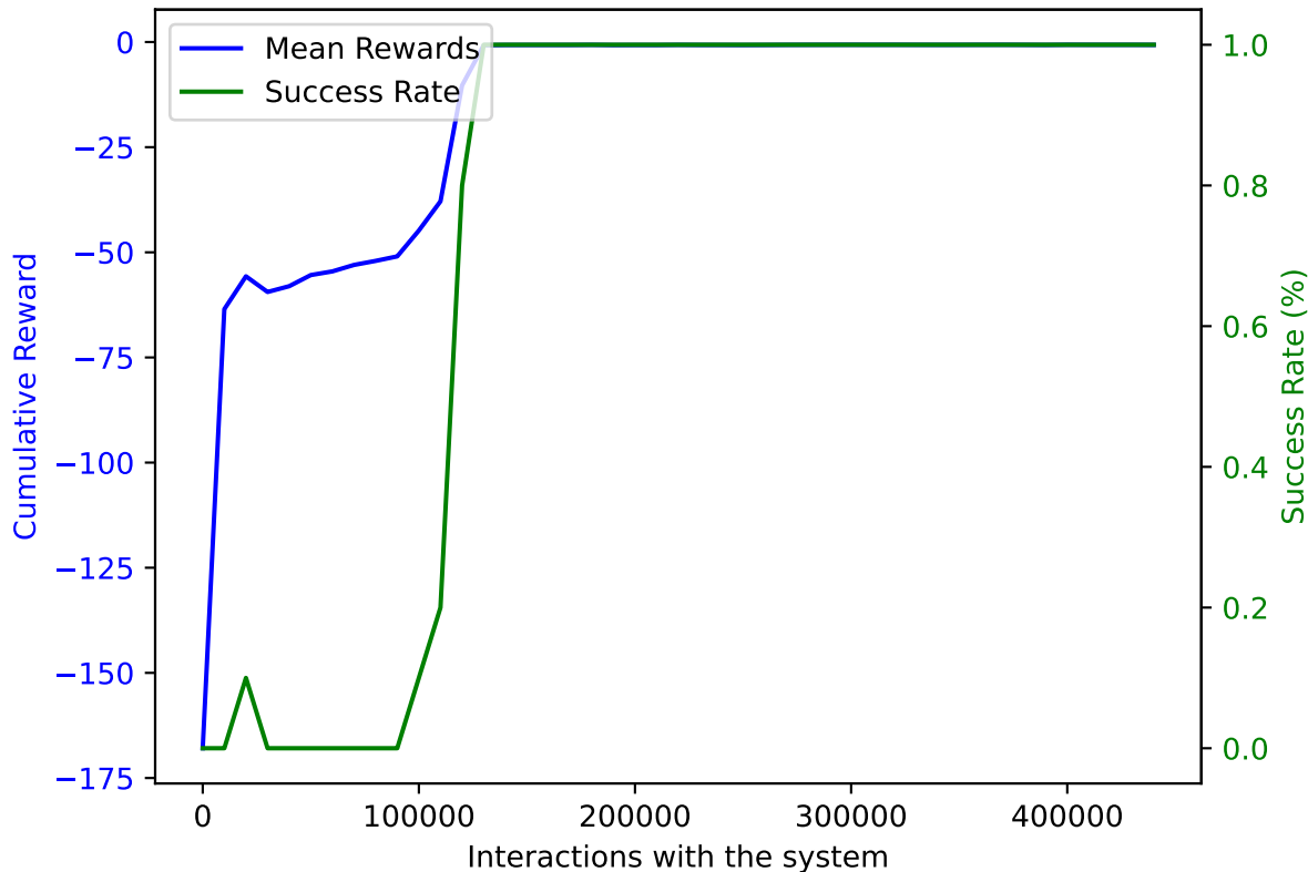
PPO on AWAKE with DoF: 5 and trained on 440000 samples averaged over 10 validation episodes
