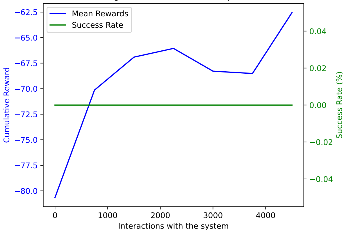
PPO on AWAKE with DoF: 5 and trained on 4500 samples averaged over 10 validation episodes
