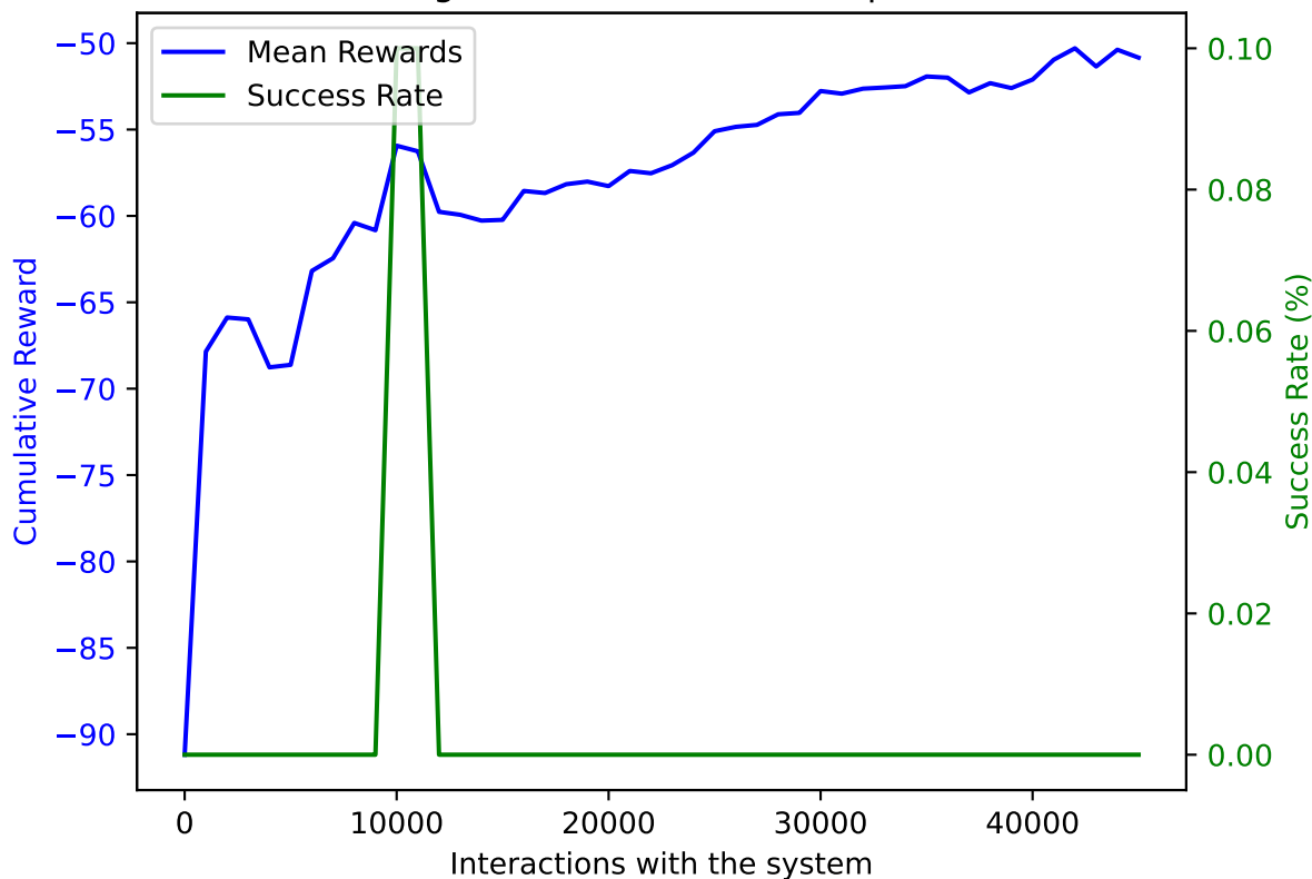
PPO on AWAKE with DoF: 5 and trained on 45000 samples averaged over 10 validation episodes
