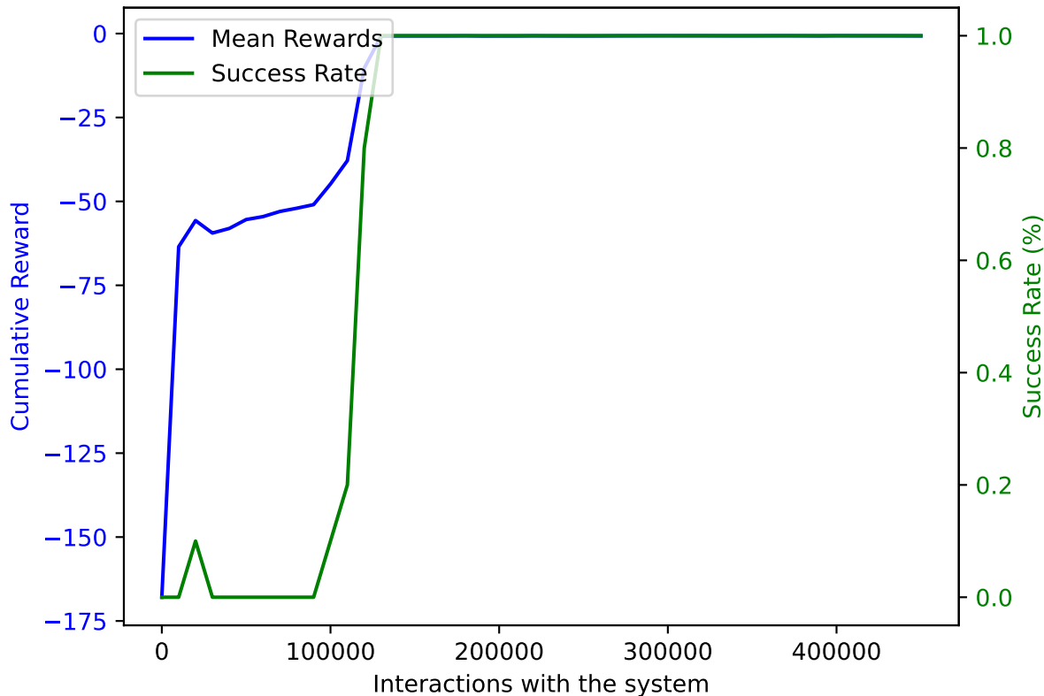
PPO on AWAKE with DoF: 5 and trained on 450000 samples averaged over 10 validation episodes
