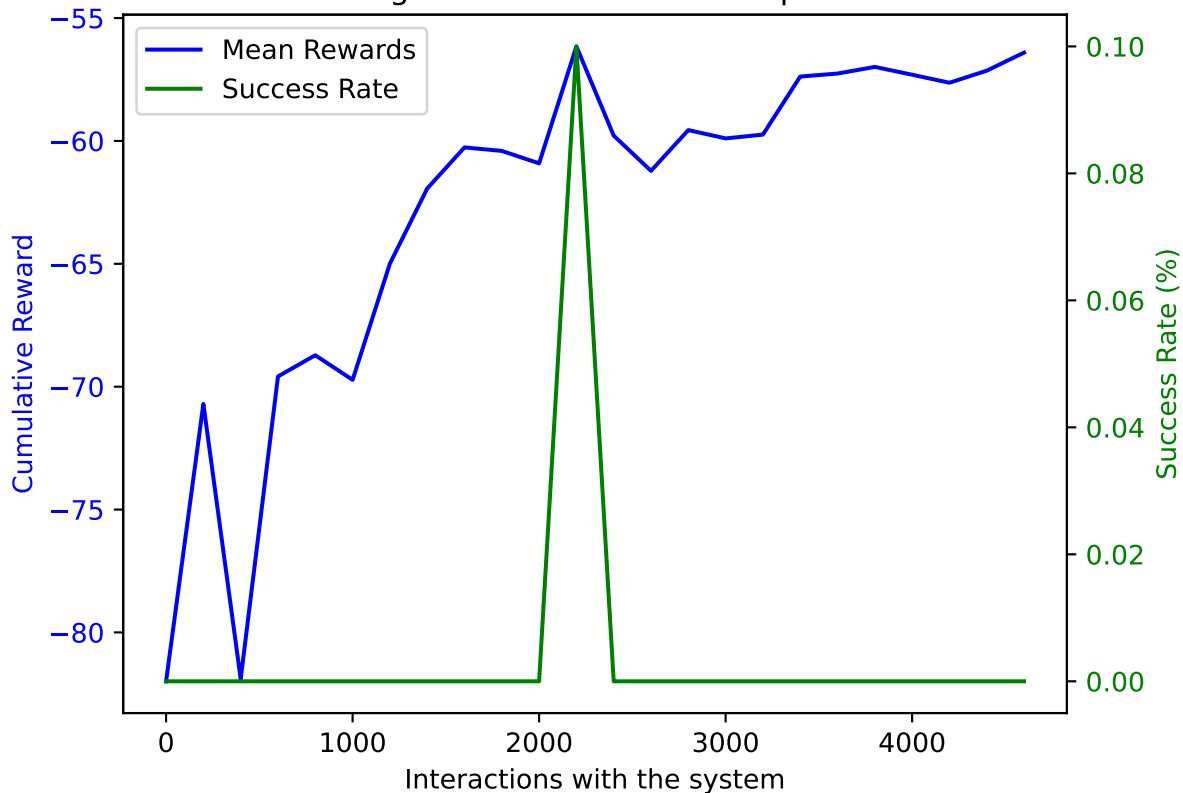
PPO on AWAKE with DoF: 5 and trained on 4600 samples averaged over 10 validation episodes
