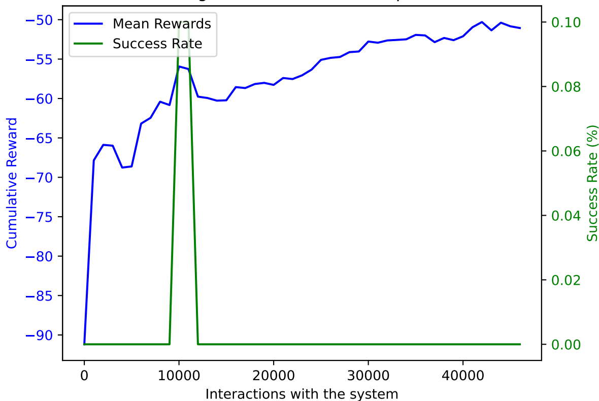
PPO on AWAKE with DoF: 5 and trained on 46000 samples averaged over 10 validation episodes
