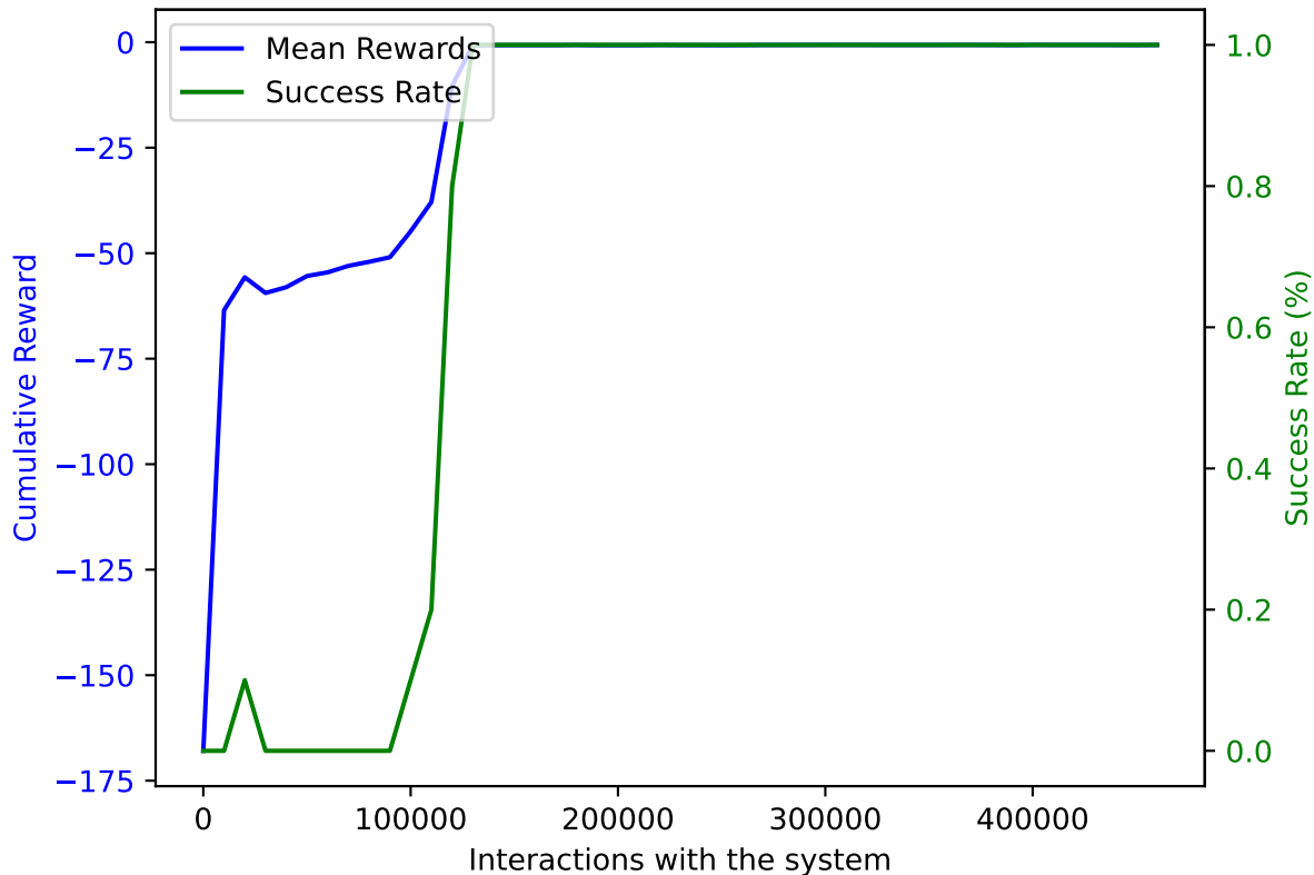
PPO on AWAKE with DoF: 5 and trained on 460000 samples averaged over 10 validation episodes
