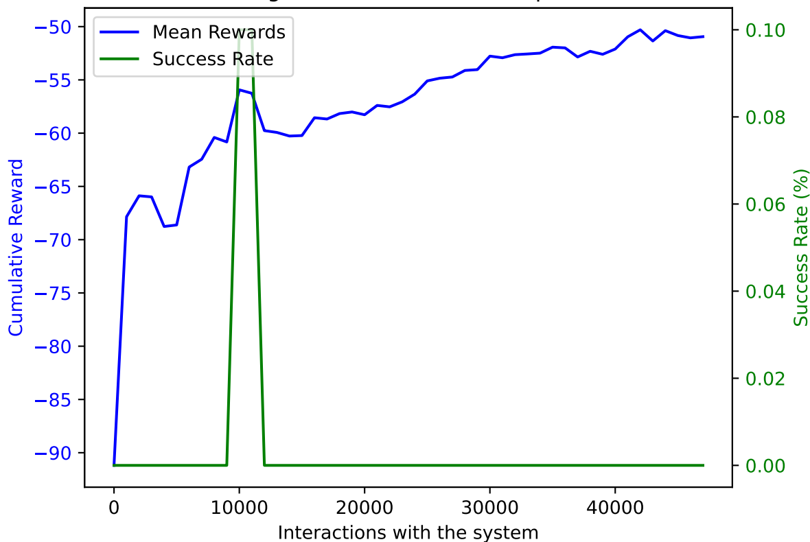
PPO on AWAKE with DoF: 5 and trained on 47000 samples averaged over 10 validation episodes
