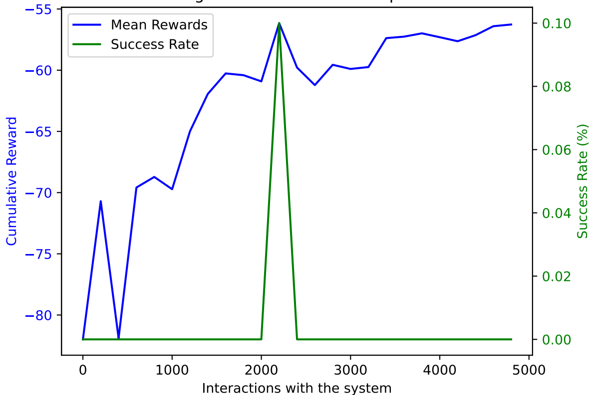
PPO on AWAKE with DoF: 5 and trained on 4800 samples averaged over 10 validation episodes
