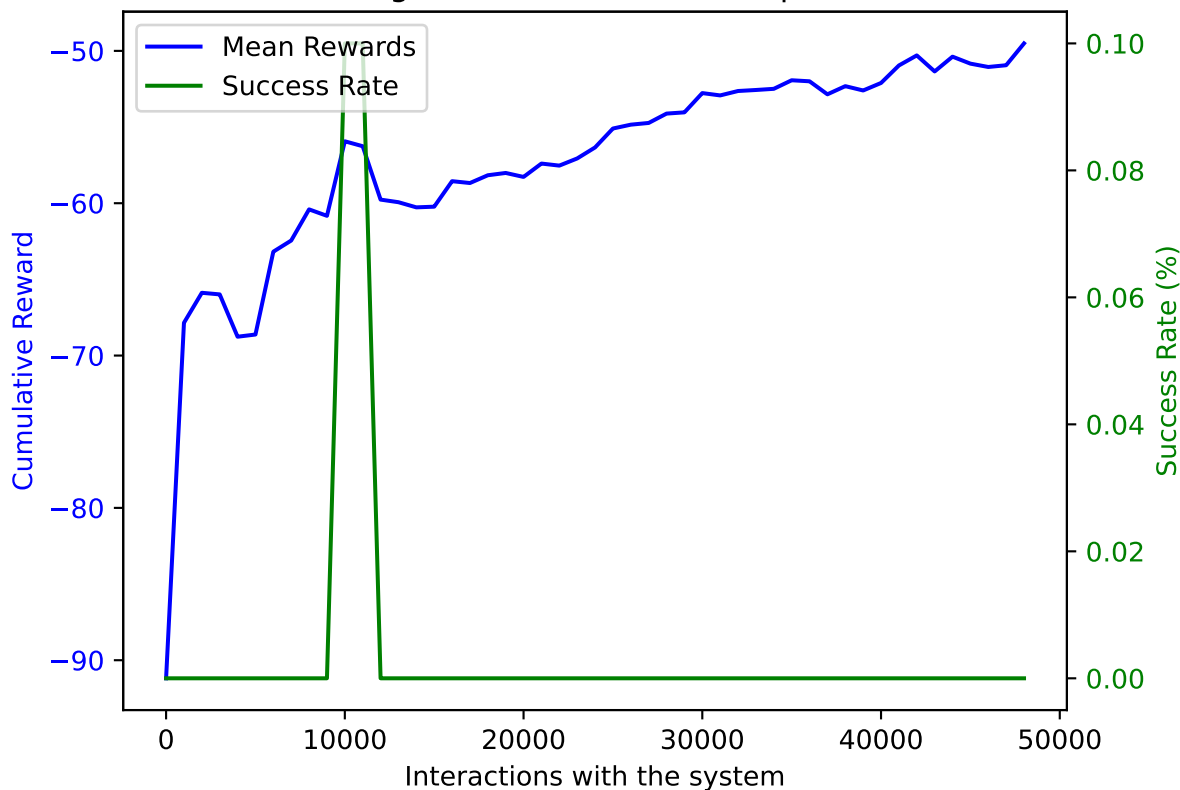
PPO on AWAKE with DoF: 5 and trained on 48000 samples averaged over 10 validation episodes
