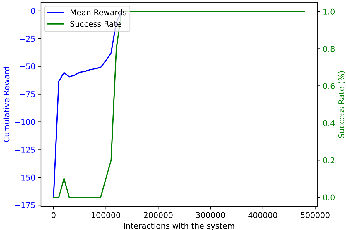
PPO on AWAKE with DoF: 5 and trained on 480000 samples averaged over 10 validation episodes
